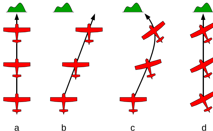
FIGURE 8.33 – Side wind
